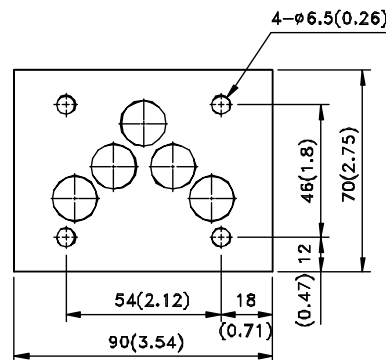
3/8" END PLATE
